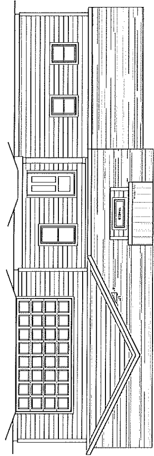
FRONT ELEVATION 1/4" = 1'-0"
