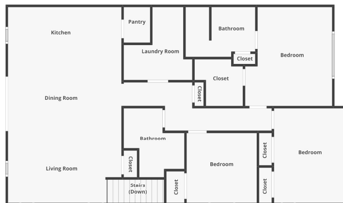
FLOOR 2
