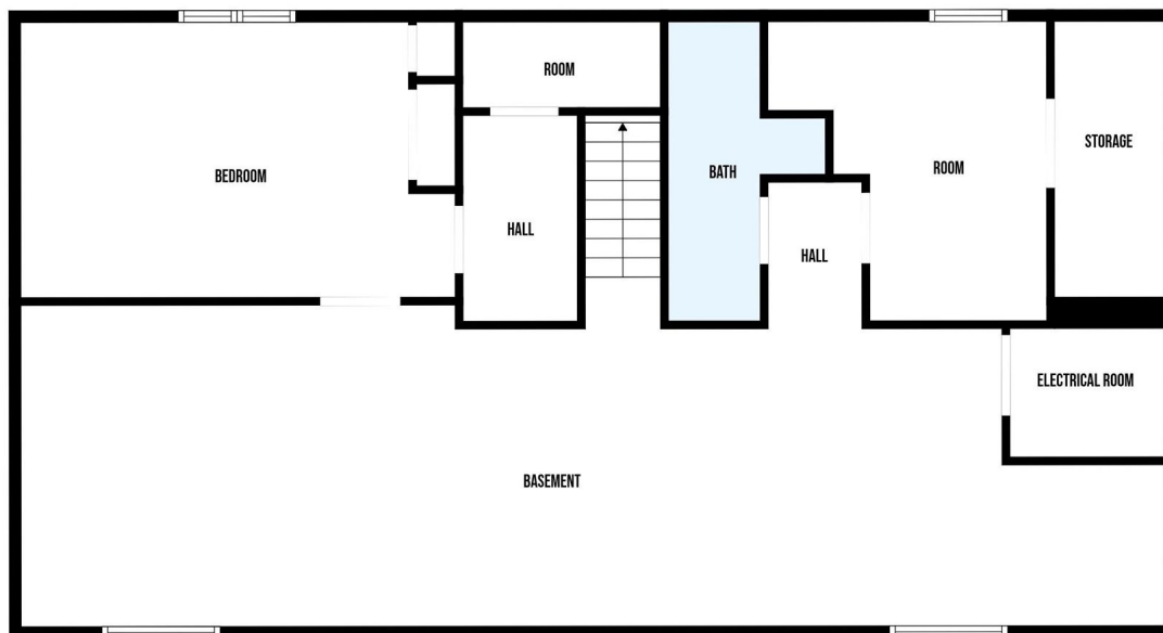
BASEMENT 1
