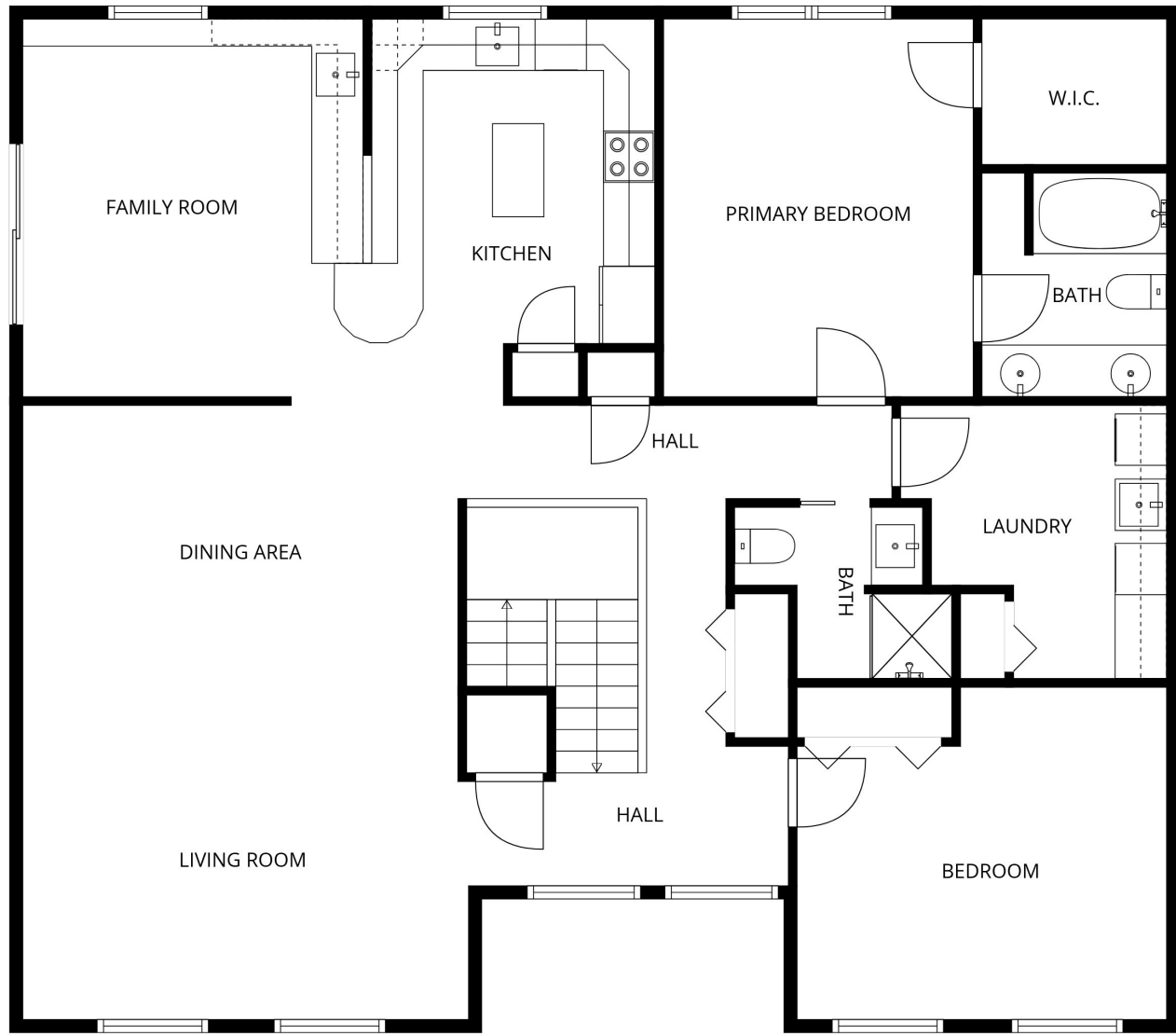
1st floor
